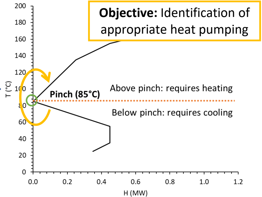
Grand Composite curve:
